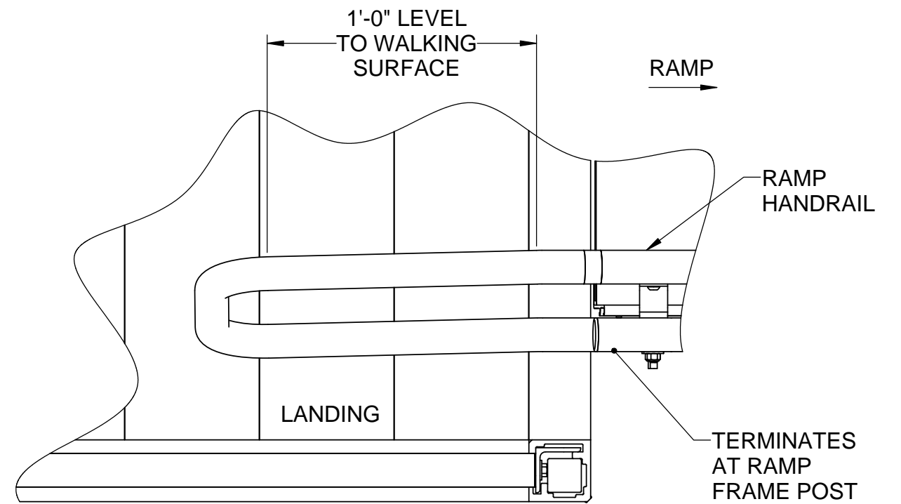
2 UPPER/LOWER HANDRAIL LOOP DETAIL 2 SCALE 1:3
