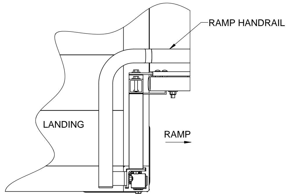
1 PLATFORM HANDRAIL TERMINATION DETAIL 2 SCALE 1:3
